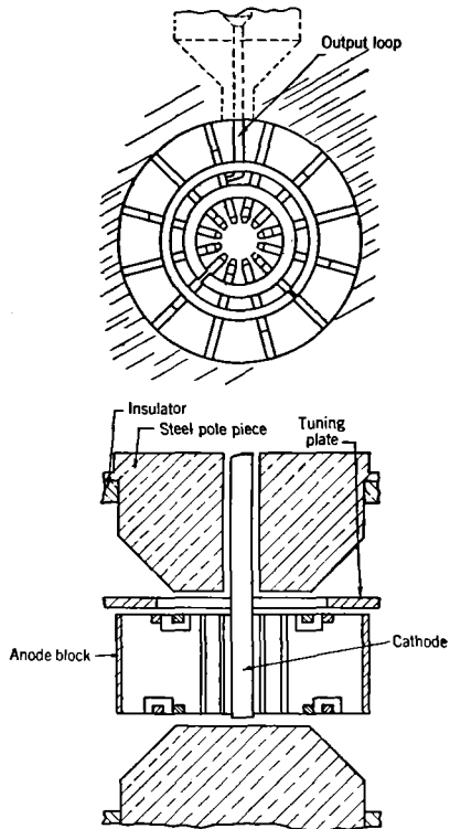
FIG. 19-35.—Cross sections of 2J41 magnetron.
